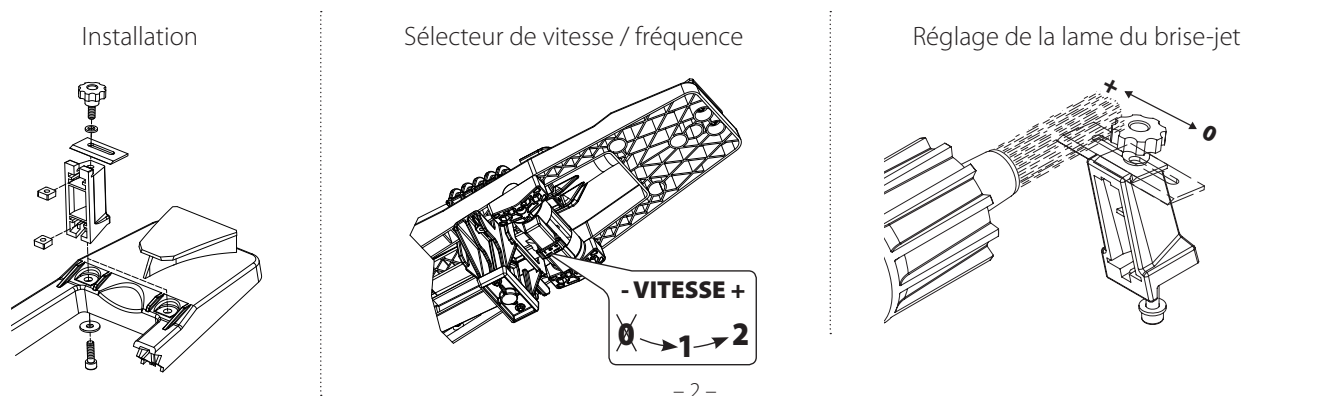
Figure 1 — Brise-jet
